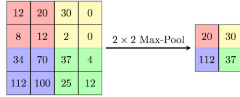
Fig. 3. Illustration of 2x2 max pooling
